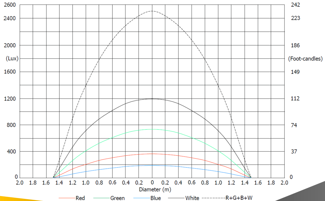
Illuminance distribution
