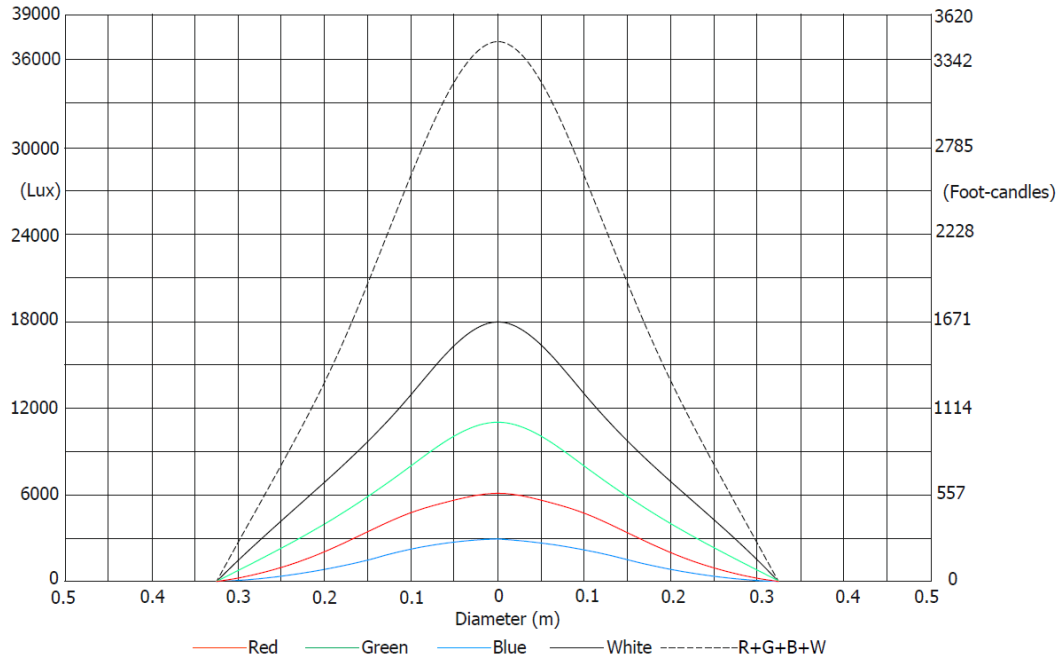
Illuminance distribution
